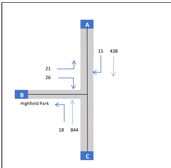
Figure 8.19: Picady Input for R117 – Highfield Park Junction AM Peak Hour – Scenario B
