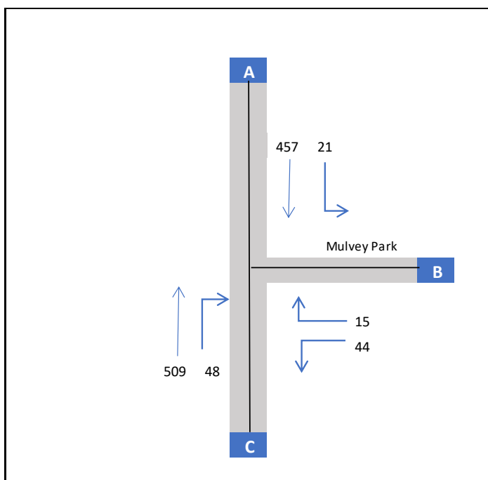
Figure 8.16: Picady Input for R117 – Mulvey Park Junction PM Peak Hour – Scenario B
