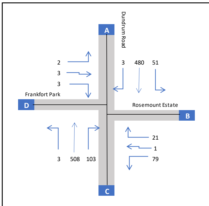
Figure 8.14: Picady Input for R117 – Frankfort Park - Rosemount Junction PM Peak Hour – Scenario B
