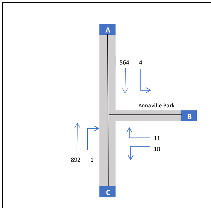
Figure 8.27: Picady Input for R117 – Annaville Park Junction AM Peak Hour - Scenario C - 2027 Opening Year with Cumulative Impact and with Proposed Development Traffic
