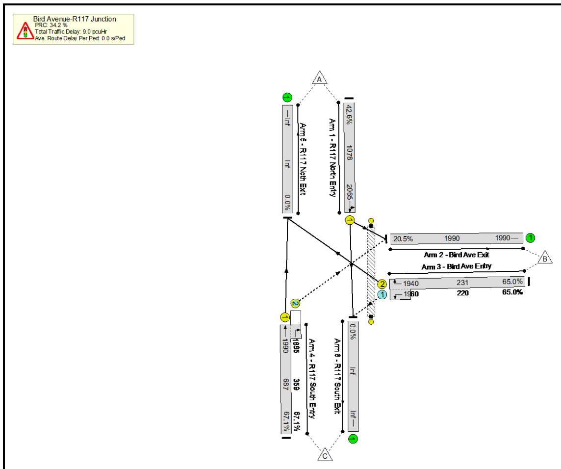
Figure 8.34: LinSig model of Bird Avenue / R117 Junction
