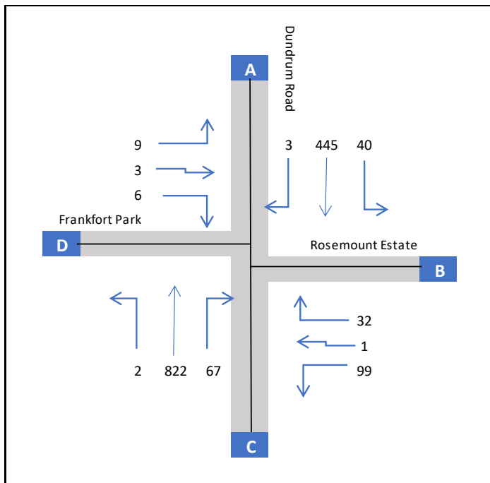
Figure 8.13: Picady Input for R117 – Frankfort Park - Rosemount Junction AM Peak Hour – Scenario B
