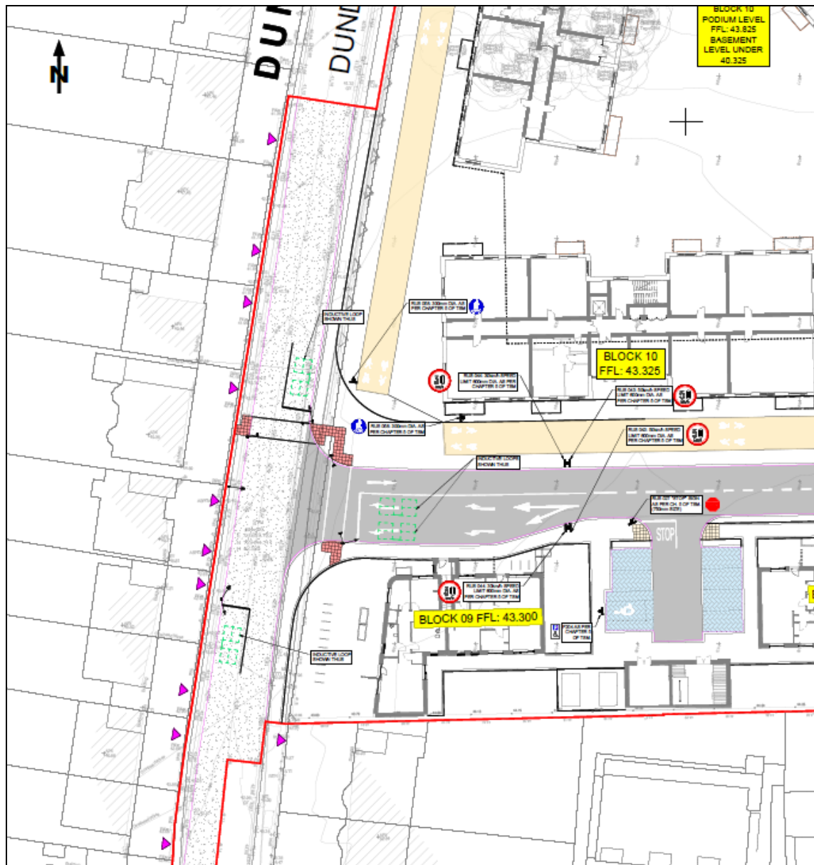
Figure 4.3: Proposed Signalised Junction (Source BMCE)
