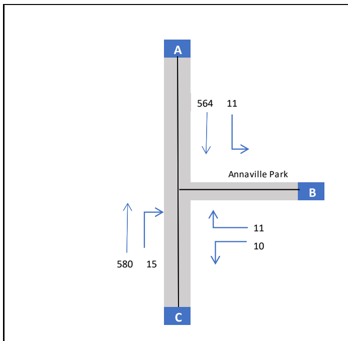
Figure 8.28: Picady Input for R117 – Annaville Park Junction PM Peak Hour - Scenario C - 2027 Opening Year with Cumulative Impact and with Proposed Development Traffic
