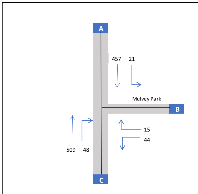
Figure 8.18: Picady Input for R117 – Annville Park Junction PM Peak Hour – Scenario B
