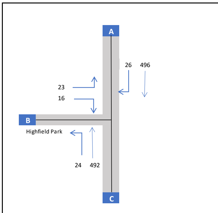
Figure 8.20: Picady Input for R117 – Highfield Park Junction PM Peak Hour – Scenario B
