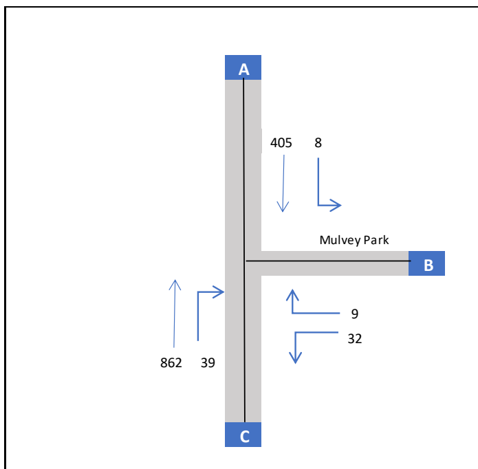
Figure 8.15: Picady Input for R117 – Mulvey Park Junction AM Peak Hour – Scenario B
